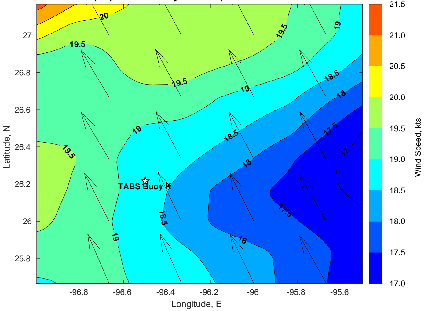
Winds (kts) for TABS Buoy K at 04-Apr-2023 12:00:00
